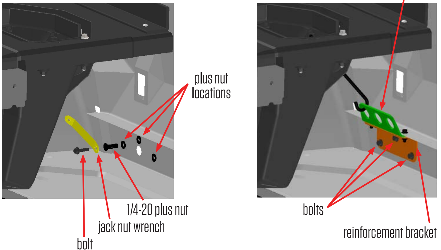
LH side reinforcement bracket shown
